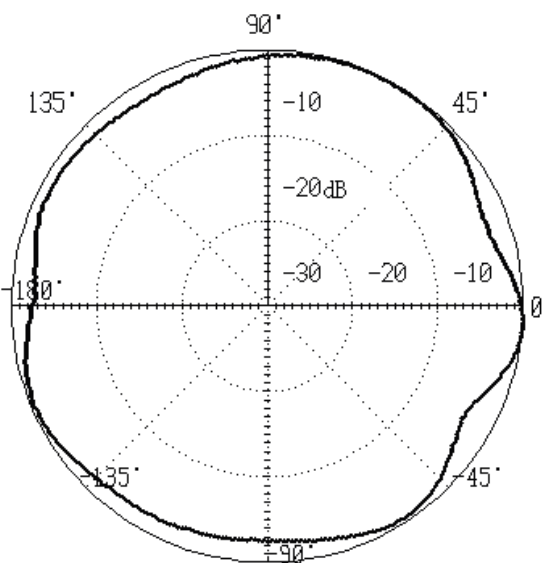
H Plane
