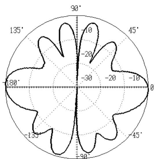
E Plane
