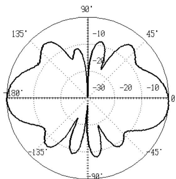
E Plane
